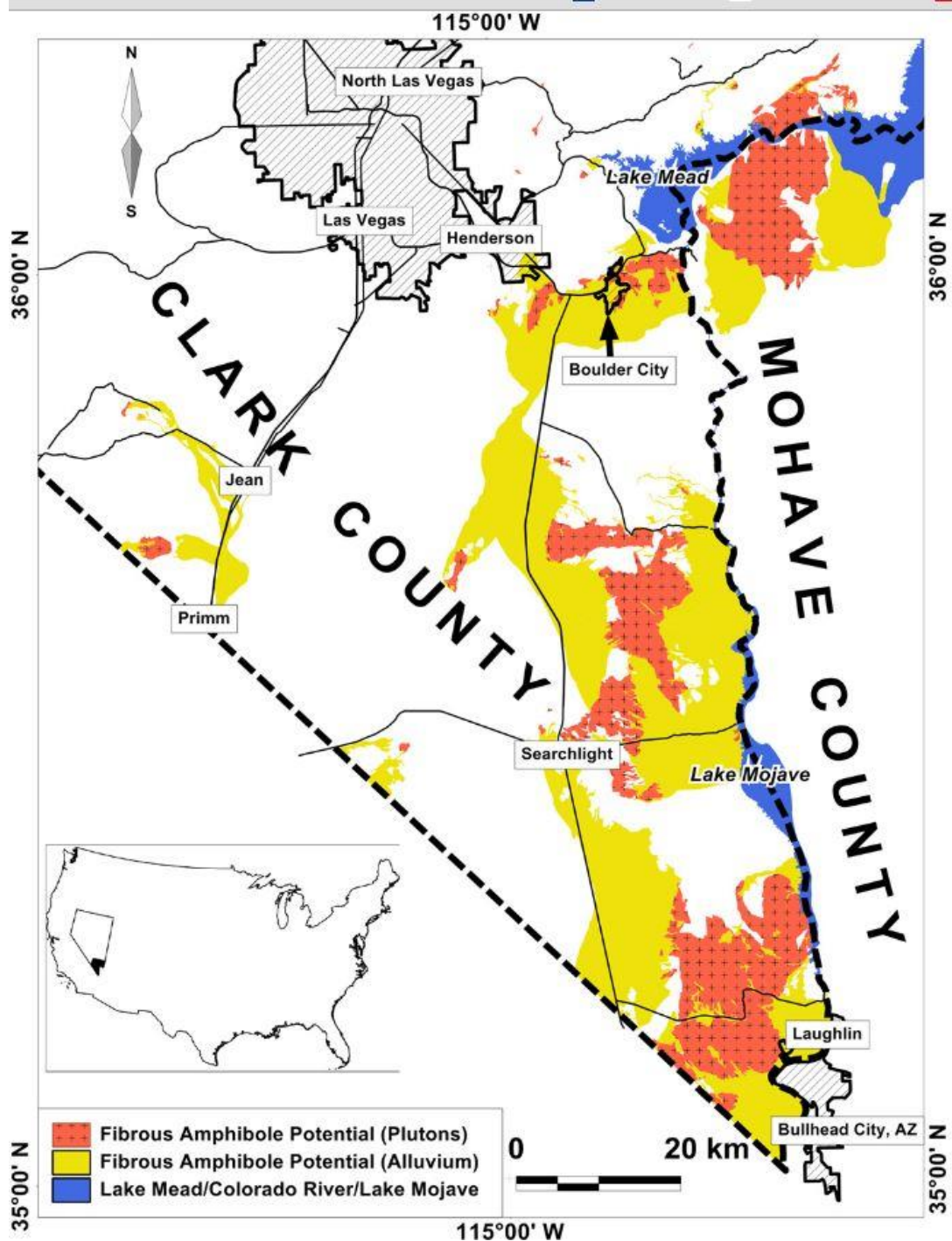
Fig 1: Predicted potential occurrence of fibrous amphiboles in Clark County, Nevada, and an area of adjacent Mohave County, Arizona, south of Lake Mead. Plutons are Miocene in age; alluvium includes deposits of Miocene to Quaternary age. Only a small portion of these mapped areas has been examined.
