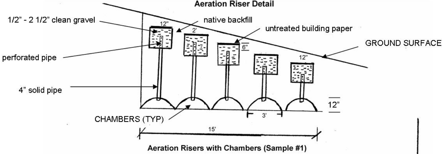
Aeration Riser Detail
